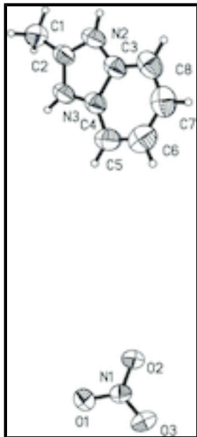
Fig. 1. The structure of the title compound showing 50% probability displacement.
